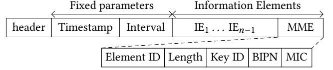
Figure 1: Beacon with a Management MIC Element (MME).
